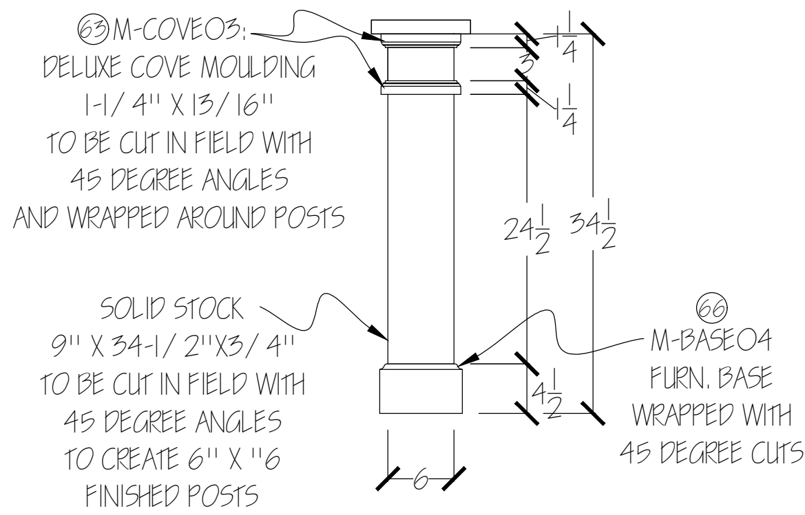
ISLAND POST DETAILS LARGE ISLAND HAS 6" X 6" POSTS AS SHOWN ABOVE SMALL ISLAND HAS 3" X 3" POSTS TO BE ASSEMBLED IDENTICAL TO THE 6" X 6" ABOVE
